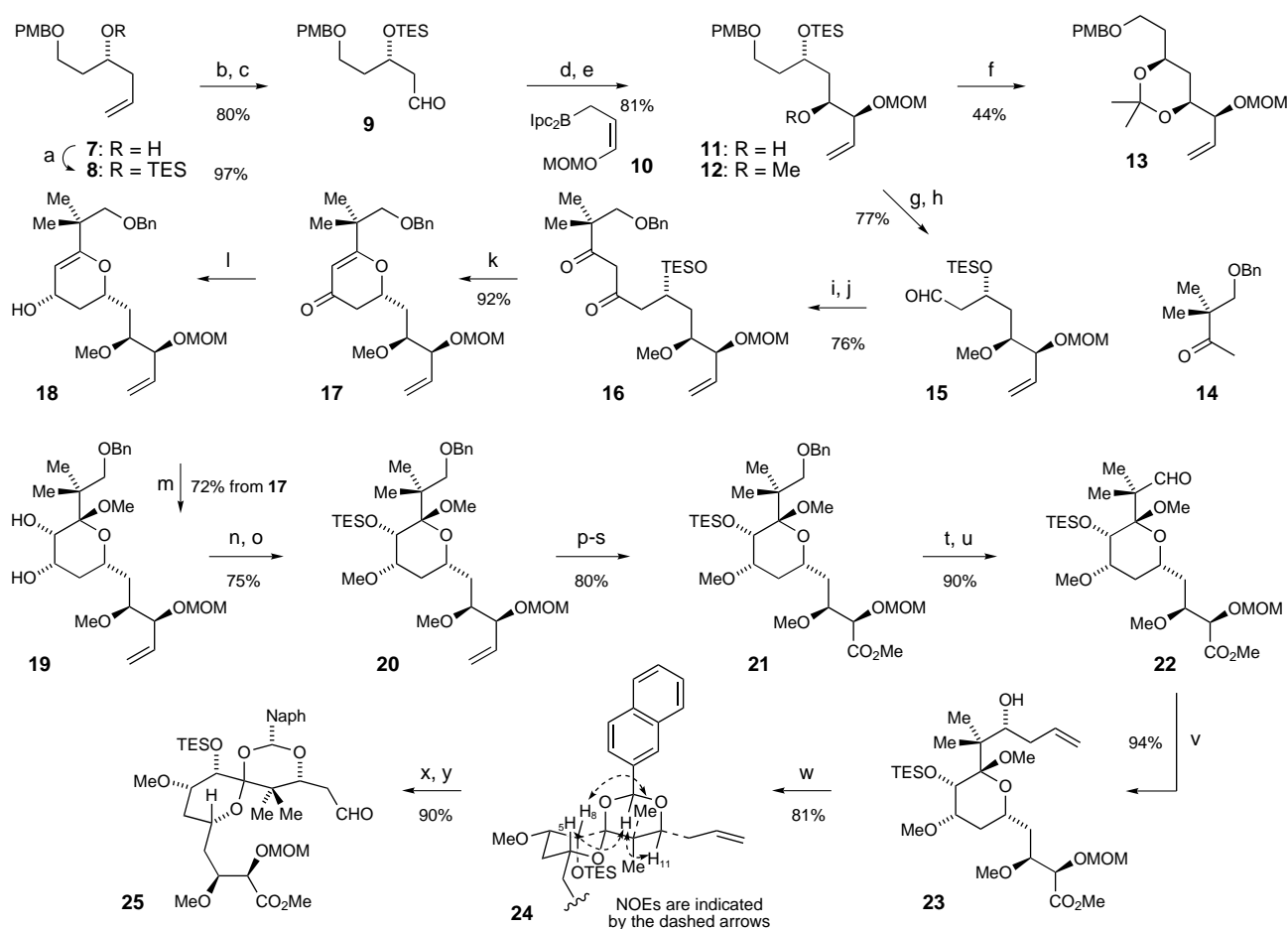
Scheme 3. a) TESOTf, 2,6-lutidine, \text{CH}_2\text{Cl}_2 (97%); b) cat. \text{OsO}_4 , NMO, acetone/ \text{H}_2\text{O} ; c) \text{Pb(OAc)}_4 , pyridine, \text{CH}_2\text{Cl}_2 (80% from 8 ); d) 10 , s\text{BuLi} , THF, -78^\circ\text{C} , 15 min, then (+)- \text{Ipc}_2\text{BOMe} , -78^\circ\text{C} , 1 h, -78 \rightarrow 0^\circ\text{C} , 1.5 h, then 9 , -95^\circ\text{C} , 3 h, slowly warm to RT; 30% \text{H}_2\text{O}_2 , NaOH, 16 h (91%); e) NaH, MeI, DMF, -5^\circ\text{C} (89%); f) PTSA, MeOH, 20 min, remove solvent, then \text{Me}_2\text{C(OMe)}_2 (44%); g) DDQ, \text{CH}_2\text{Cl}_2/\text{H}_2\text{O} , 0^\circ\text{C} (88%); h) \text{py-SO}_3 , \text{Et}_3\text{N} , DMSO, \text{CH}_2\text{Cl}_2 , 0^\circ\text{C} (87%); i) 14 , LDA, THF, -78^\circ\text{C} , then 15 , -78^\circ\text{C} (94%); j) Dess–Martin periodinane, \text{CH}_2\text{Cl}_2 , -10^\circ\text{C} (81% based on recovered starting material); k) PTSA, PhMe, RT (92%); l) \text{NaBH}_4 , \text{CeCl}_3 \cdot 7\text{H}_2\text{O} , MeOH, -30^\circ\text{C} ; m) m CPBA, \text{NaHCO}_3 , \text{CH}_2\text{Cl}_2/\text{MeOH} , 0^\circ\text{C} (72%, two steps); n) t\text{BuOK} , MeI, THF, 0^\circ\text{C} ; o) TESOTf, 2,6-lutidine, \text{CH}_2\text{Cl}_2 (75% from 19 ); p) cat. \text{OsO}_4 , NMO, acetone/ \text{H}_2\text{O} ; q) \text{Pb(OAc)}_4 , pyridine, \text{CH}_2\text{Cl}_2 ; r) \text{NaClO}_2 , \text{NaH}_2\text{PO}_4 , 2-Me-2-butene, t\text{BuOH}/\text{H}_2\text{O} ; s) \text{CH}_2\text{N}_2 , \text{Et}_2\text{O} , 0^\circ\text{C} (80% from 20 ); t) \text{H}_2 , Pd/C (10%), MeOH (quant.); u) \text{py-SO}_3 , \text{Et}_3\text{N} , DMSO, \text{CH}_2\text{Cl}_2 , 0^\circ\text{C} (90%); v) allyl \text{BEt}_2 , \text{Et}_2\text{O} , -10^\circ\text{C} (94%); w) TESOTf, 2-naphthaldehyde, -78^\circ\text{C} , then 2,6-lutidine, TESOTf, 0^\circ\text{C} (81%); x) cat. \text{OsO}_4 , NMO, acetone/ \text{H}_2\text{O} ; y) \text{NaIO}_4 on silicagel, \text{CH}_2\text{Cl}_2 (90% from 24 ). PMB = p -methoxybenzyl, TES = triethylsilyl, Tf = trifluoromethane sulfonate, NMO = 4-methylmorpholine- N -oxide, MOM = methoxymethyl, Ipc = isopinocampheyl, DDQ = 2,3-dichloro-5,6-dicyano-1,4-benzoquinone, LDA = lithium diisopropylamide, PTSA = p -toluenesulfonic acid, m CPBA = m -chloroperbenzoic acid.
