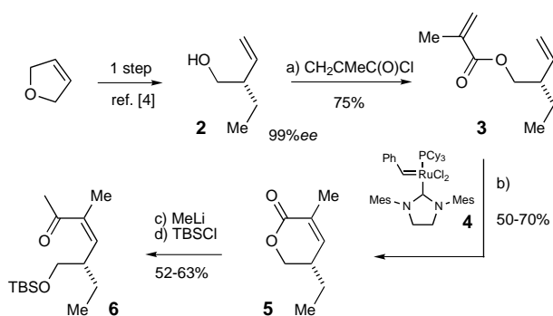
Scheme 2. a) \text{CH}_2\text{CMeC(O)Cl} , i\text{Pr}_2\text{NEt} , DMAP, \text{CH}_2\text{Cl}_2 (75%); b) 10 mol % 4 , \text{CH}_2\text{Cl}_2 (0.0025 M), reflux, 17 h (50–70% + 20% dimer derived from 3 ); c) MeLi, THF, -78^\circ\text{C} ; or \text{Me}_3\text{SiCH}_2\text{Li} , pentane, -78^\circ\text{C} ; d) TBSCl, imidazole, DMAP, DMF (52–63% from 5 ). DMAP = 4-dimethylaminopyridine, TBS = tert -butyldimethylsilyl.
