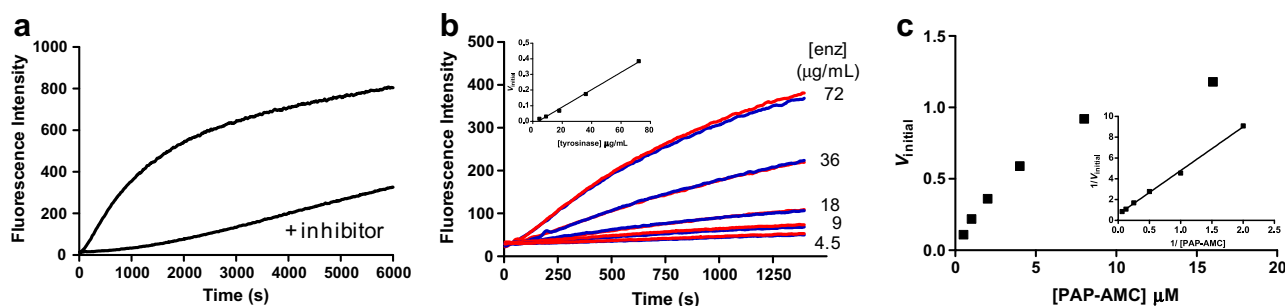
Figure 1. Fluorescence monitoring of the mushroom tyrosinase-catalyzed oxidation of PAP-AMC . (a) Oxidation of PAP-AMC in the presence or absence of 0.2 M kojic acid. (b) Reactions in the presence of varying concentrations of tyrosinase. Duplicate experiments are shown. Inset: plot of initial rate versus [tyrosinase]. (c) Initial rates as a function of [PAP-AMC]. Inset: Lineweaver–Burk plot. For all experiments, \lambda_{\text{excitation}} = 350 \text{ nm} ; \lambda_{\text{emission}} = 460 \text{ nm} .
