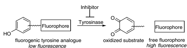
Scheme 1. Strategy for fluorogenic reporter of tyrosinase activity.
